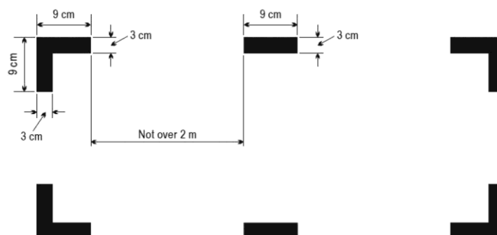
Marking of break-in points
